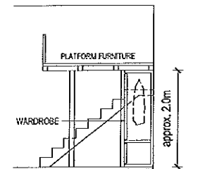
SECTION Applicable to Type A2aL only
